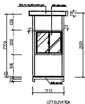
LEFT ELEVATION
