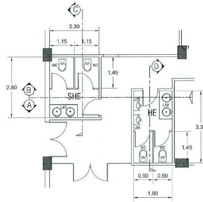
MENS & WOMENS TOILET TYPICAL PLAN SCALE 1:100M
