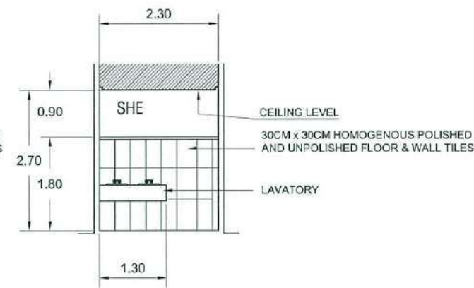
WOMENS TOILET SECTION A-A SCALE 1:100M
