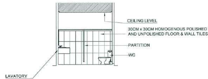
WOMENS TOILET SECTION C-C SCALE 1:100M
